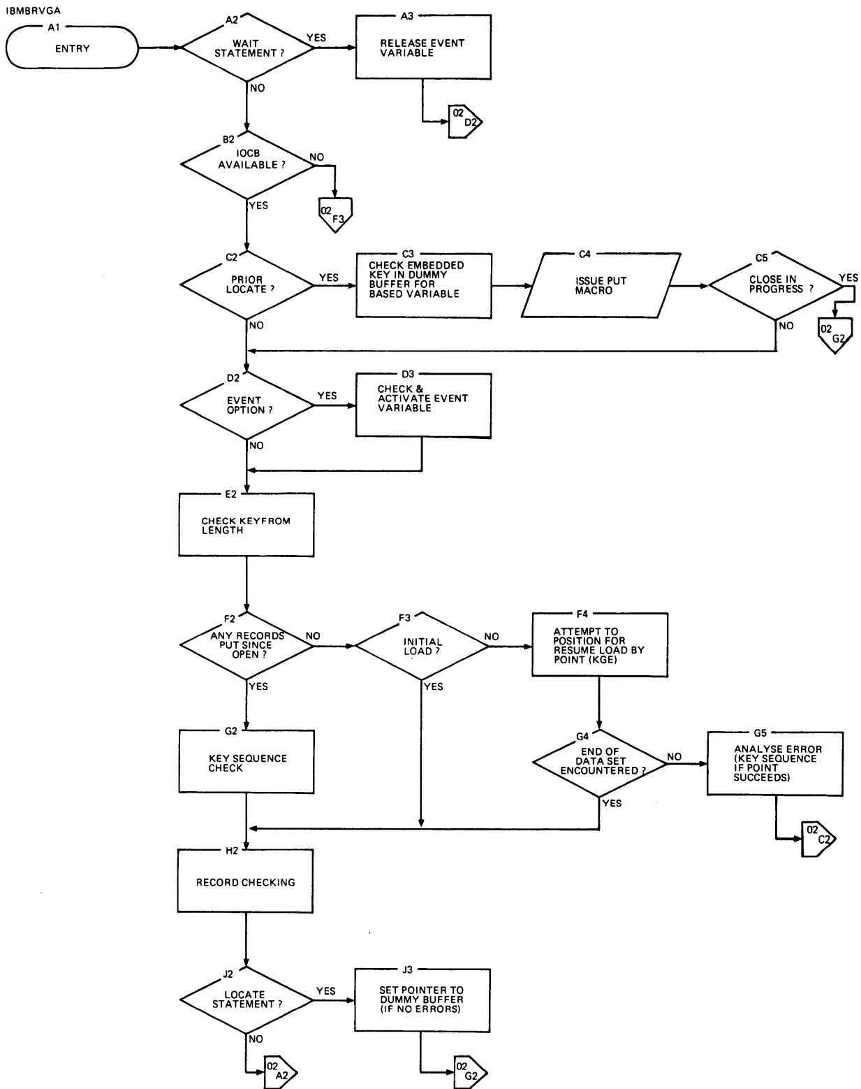
|Chart DRVT. KSDS Sequential output transmitter (part 1 of 2)
