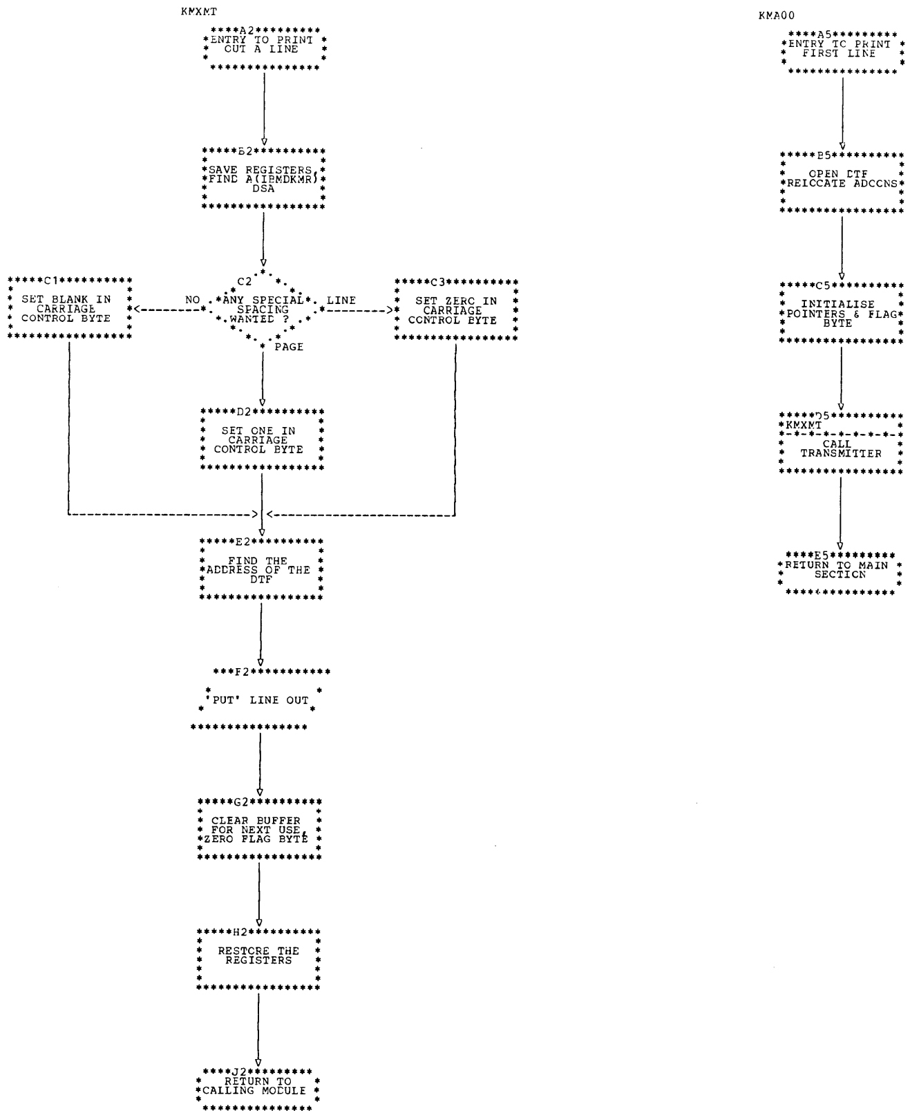
Chart DKMR. Dump control module (part 2 of 3)
