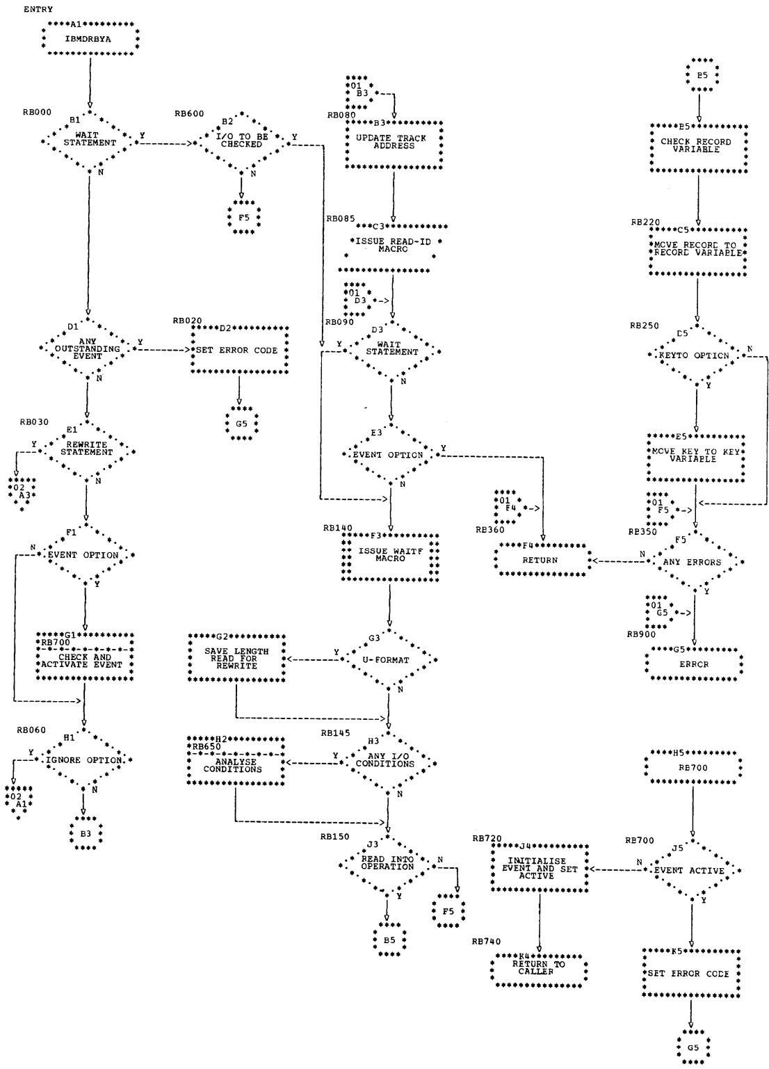
Chart DREY. Regional(3) sequential unbuffered input/update transmitter (part 1 of 2)
