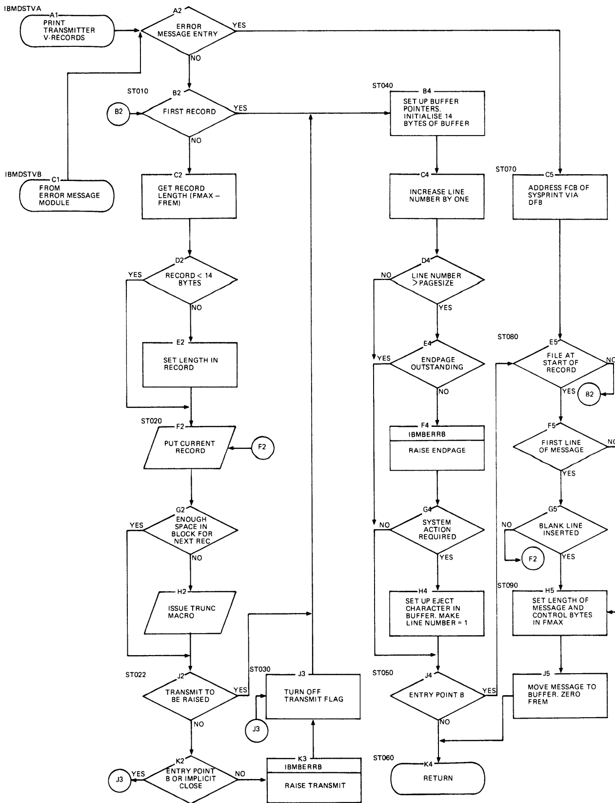
Chart DSTV. Stream print V-format transmitter
